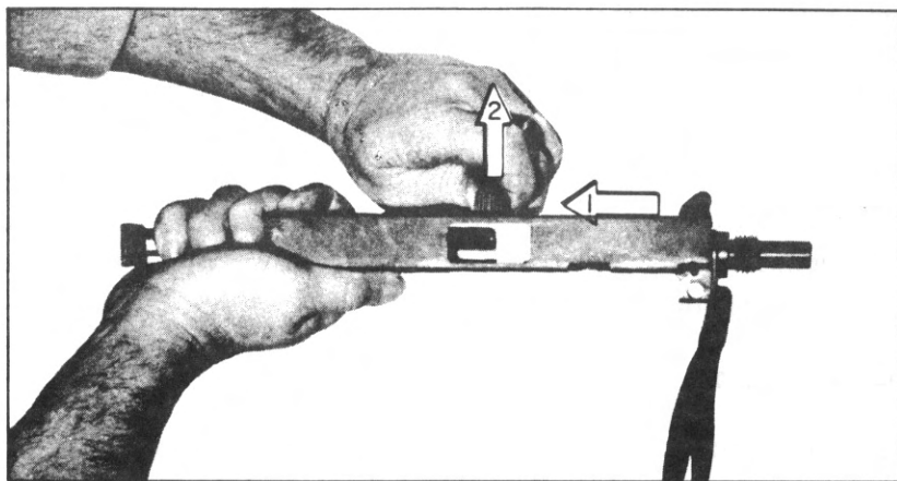
FIG. 15 Removing Cocking Handle
