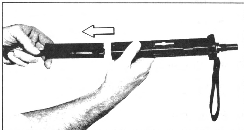
FIG. 16 Bolt Remover from Rear of Receiver
