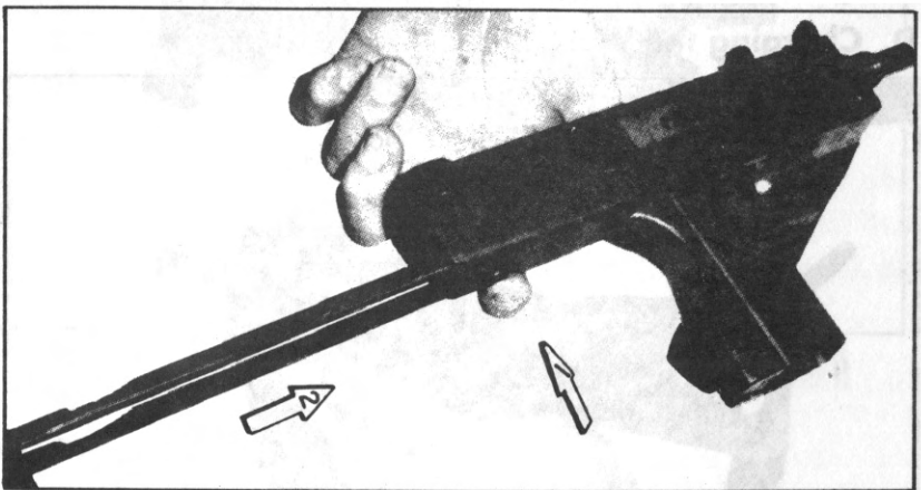
FIG. 6 Retract Wire Form Stock
