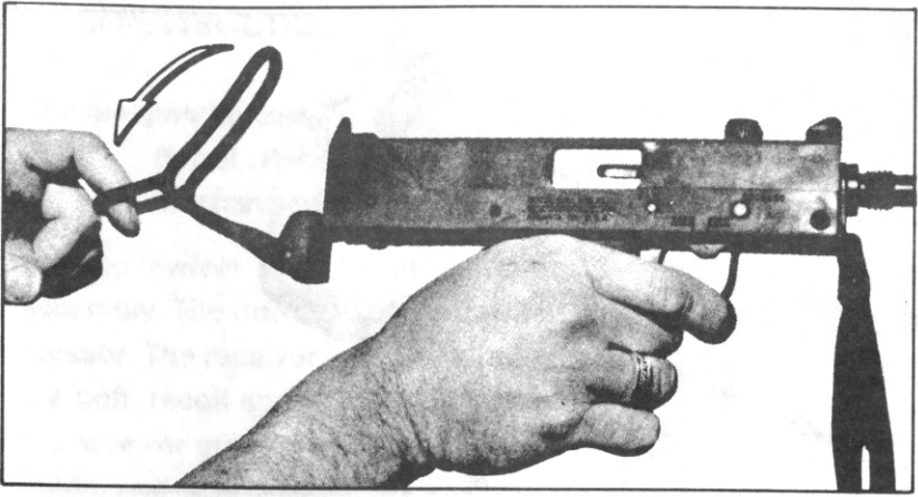
FIG. 3 Pull Down On Wire Form Butt
