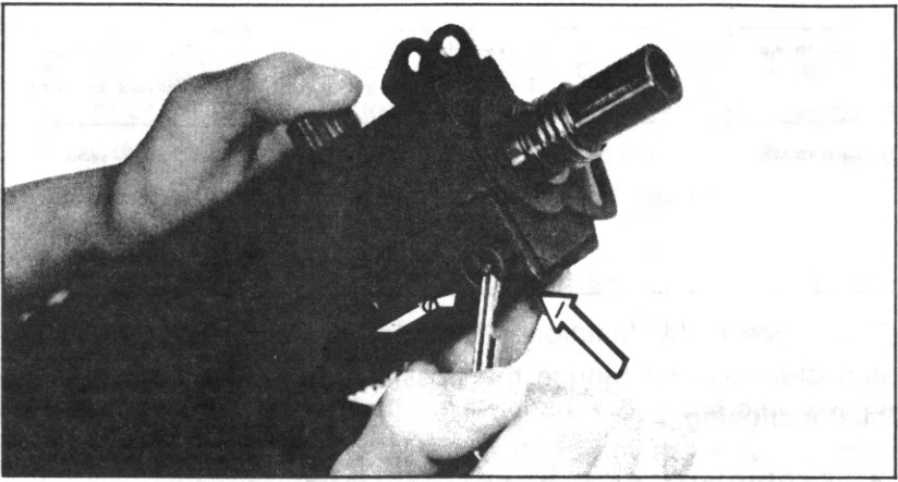
FIG. 13 Removing Pin Securing Receiver Group
